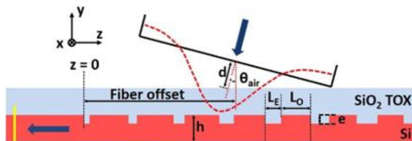
Figure 6: Grating Coupler (side view). Figure from Riccardo Marchetti et al., "High-efficiency grating-couplers: demonstration of a new design strategy". Nature 2017.
