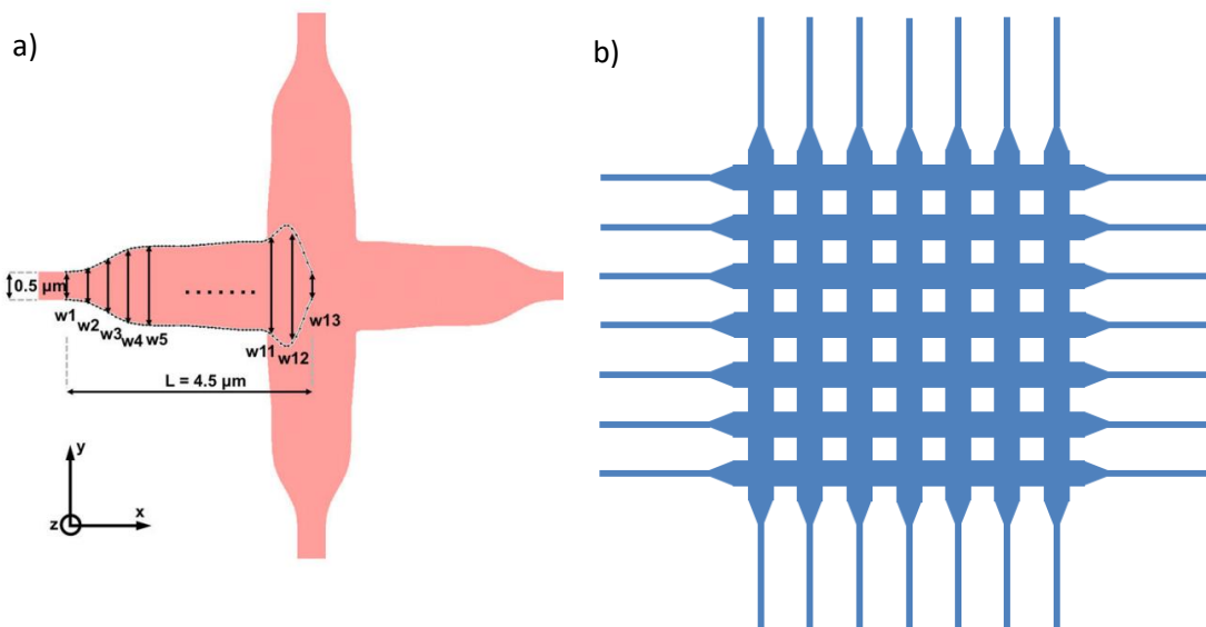
Figure 7: (a) A 2 waveguide crossing with mode expanders is shown (Ma, Yangjin, et al. "Ultralow loss single layer submicron silicon waveguide crossing for SOI optical interconnect." Optics express 21.24 (2013): 29374-29382). (b) A Network of a 7x7 WG crossing is illustrated (Zhang, Yang, et al. "Ultralow-loss silicon waveguide crossing using Bloch modes in index-engineered cascaded multimode-interference couplers." Optics letters 38.18 (2013): 3608-3611).
