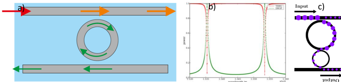
Figure 2: (a) The ring resonator structure is illustrated. (b) The expected transmission and reflection coefficients over a variation of the wavelength. (c) An illustration of two cascaded ring resonators.
