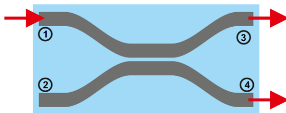
Figure 1: An illustration of a directional coupler.
