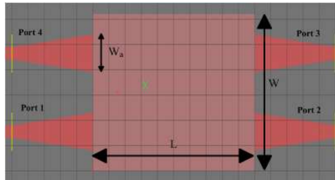
Figure 5: Multimode interferometer 2x2 configuration. (Image Source: https://optics.ansys.com/hc/en-us/articles/360042323574-Circuit-simulation-incorporating-component-level-results )
